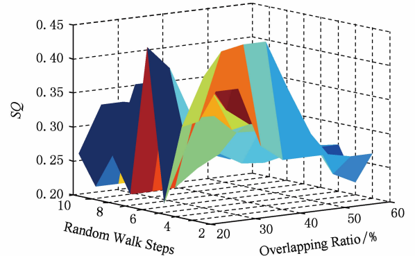
Fig. 7 The SQ of QLSP network.
