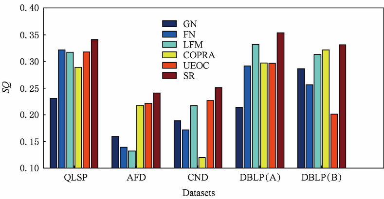
Fig. 13 The histogram of SQ for different classical algorithms.
