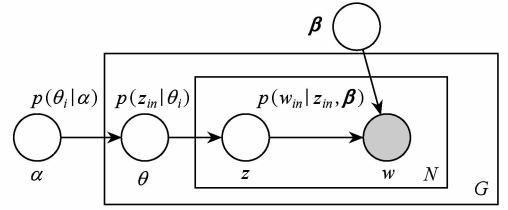
Fig. 1 The LDA plate model.
