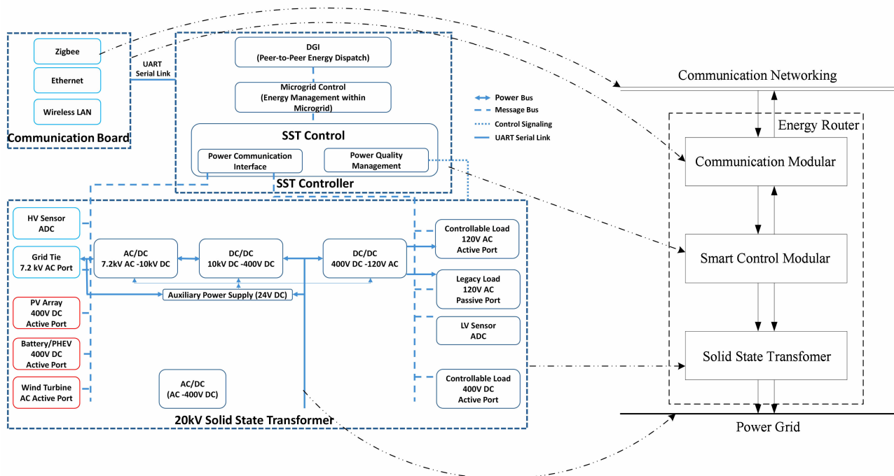
Fig. 8 Layered architecture of power energy routers.
