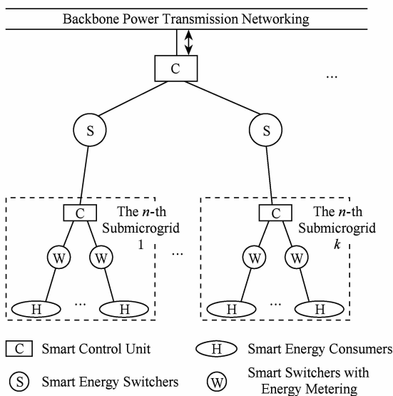
Fig. 5 The tree structure of energy Internet.
