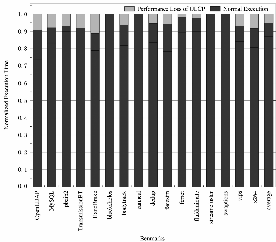
Fig. 9 The normalized execution time through replaying the traces with and without ULCs.
