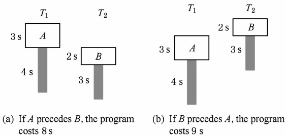
Fig. 3 The performance fluctuation arising from two possible lock interleavings.
