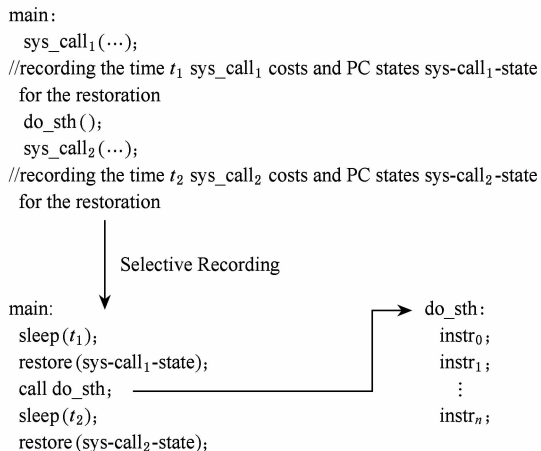
Fig. 2 The technical features of selective recording technique.
