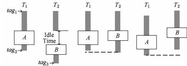
Fig. 7 Two possible schedules after the optimization for the performance measurement of each ULC.
