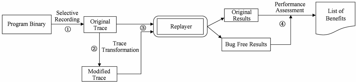
Fig. 4 The architecture of PerfPlay.
