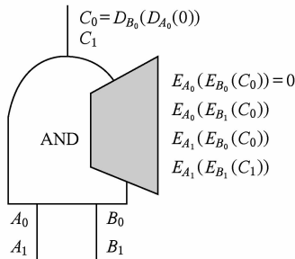
Fig. 4 Garbled computation with 3 rows.
