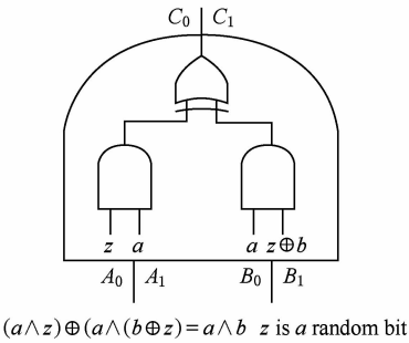
Fig. 7 The technic of Half-Gate. 图 7 Half-Gate 技术
