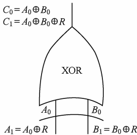
Fig. 2 The technic of Free-XOR.
