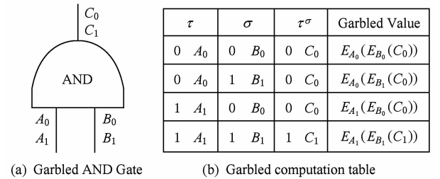
Fig. 1 The garbled AND Gate and garbled computation table in Yaos' scheme. 图 1 Yao 方案与门混乱电路及混乱表
