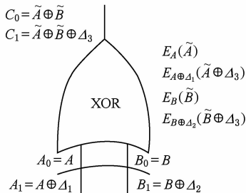
Fig. 3 The technic of FleXOR.
