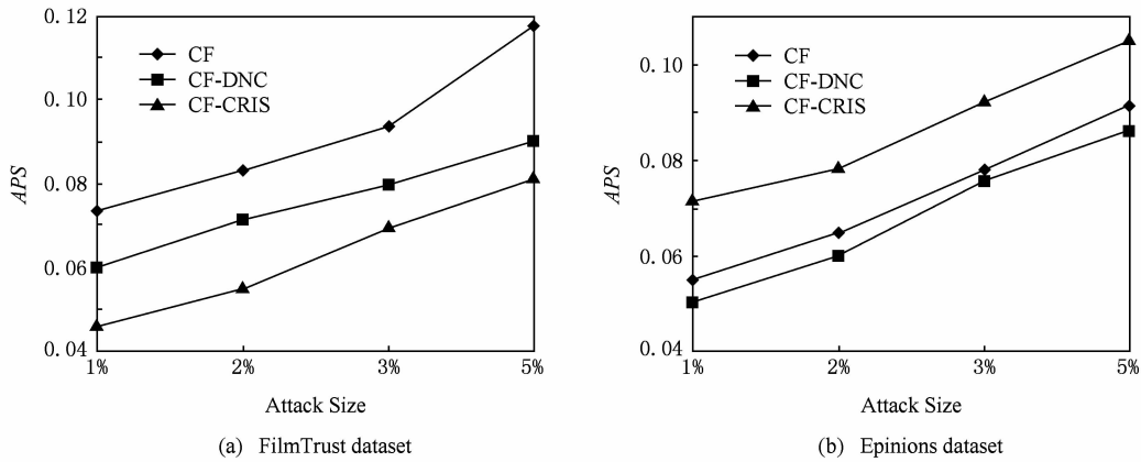
Fig. 6 Comparison of APS with 5% filling size. 图 6 5%填充规模时平均预测偏差(APS)对比
