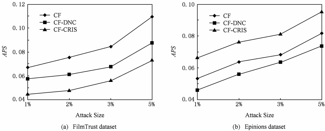
Fig. 5 Comparison of APS with 3% filling size. 图 5 3%填充规模时平均预测偏差(APS)对比
