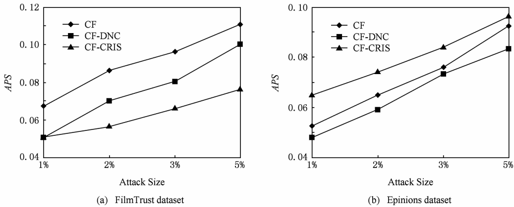
Fig. 7 Comparison of APS with 10% filling size. 图 7 10%填充规模时平均预测偏差(APS)对比
