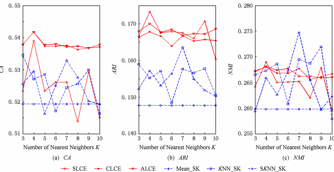
Fig. 4 The performance of different algorithms with respect to different number of neighborhood on the Automobile dataset.
