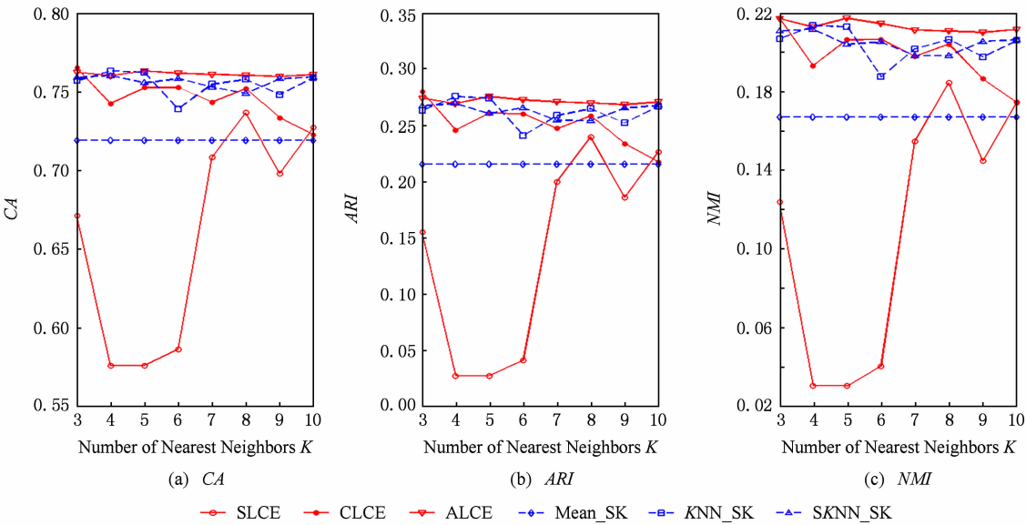
Fig. 3 The performance of different algorithms with respect to different number of neighborhood on the Credit Approval dataset.
