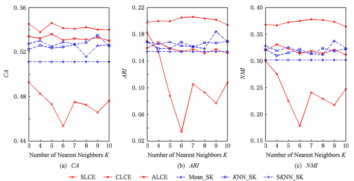
Fig. 8 The performance of different algorithms with respect to different number of neighborhood on the Glass dataset.
