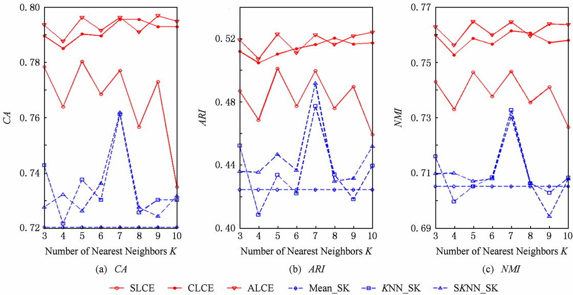
Fig. 5 The performance of different algorithms with respect to different number of neighborhood on the Sponge dataset.
