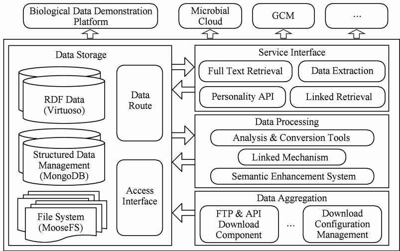
Fig. 2 Scientific data fusion management and service architecture.
