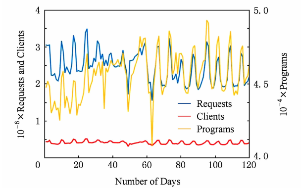
Fig. 1 Number of requests, active clients, and distinct programs requested over 120 days.
