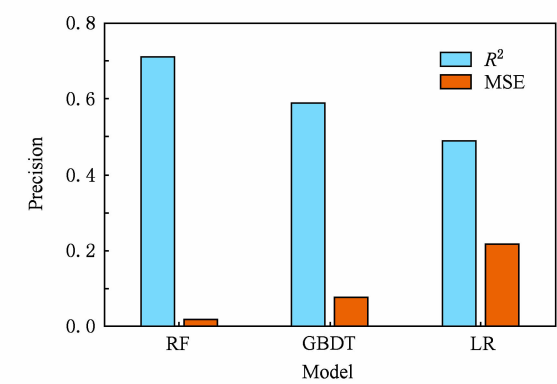
Fig. 6 Comparison of precision between RF, LR and GBDT.
