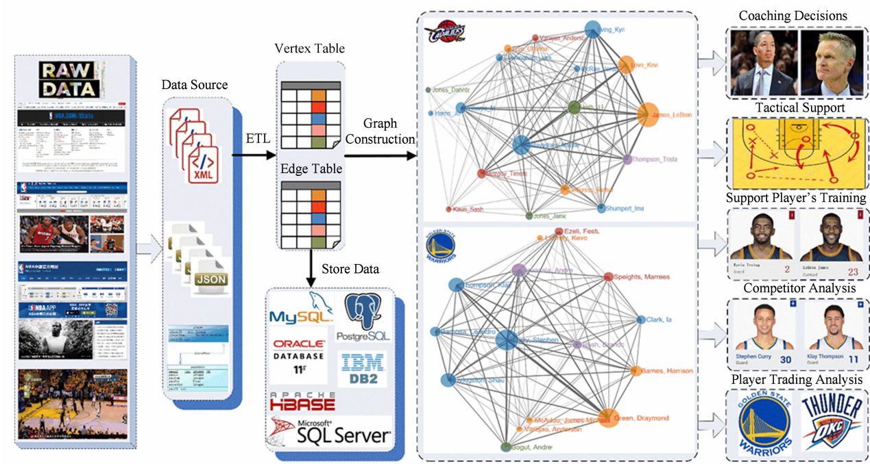
Fig. 2 The construction and application framework of passing network diagram. 图 2 传球网络图构建及应用框架流程图
