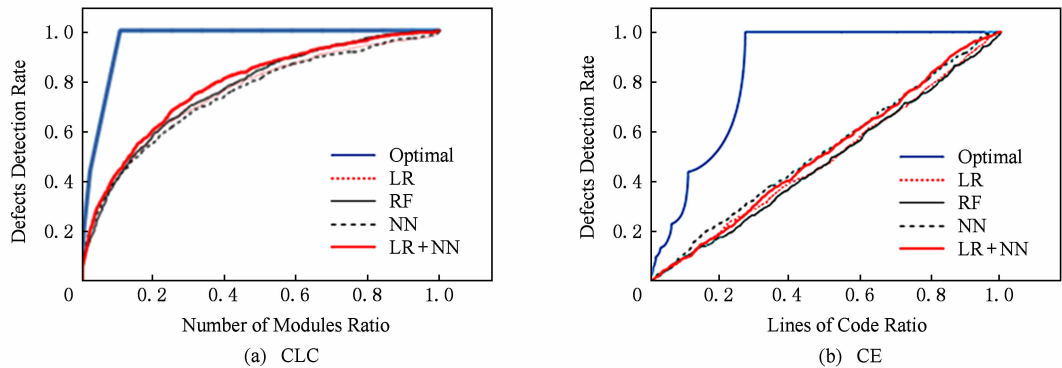
Fig. 4 Results of combined machine learning model (File 2.0 as training set, File 2.1 as testing set) 图 4 组合机器学习模型的部分预测结果(训练集为 File 2.0、测试集为 File 2.1)
