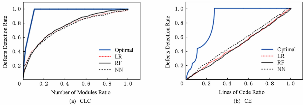
Fig. 3 Results of different machine learning model (File 2.0 as training Set, File 2.1 as testing Set) 图 3 不同机器学习模型的部分预测结果(训练集为 File 2.0、测试集为 File 2.1)
