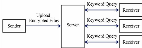
Fig. 4 One-to-many mode searchable encryption
