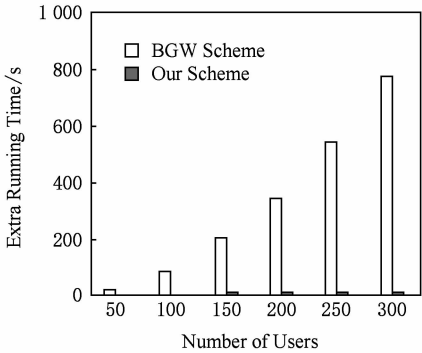
Fig. 4 Time cost vs the number of users between BGW and our scheme
