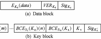
Fig. 3 The cloud data format when lazy revocation is introduced
