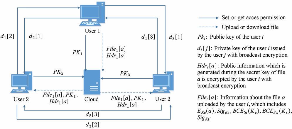
Fig. 1 Interactive processes between the user and the cloud
