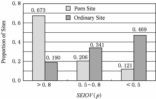
Fig. 3 SEIOV(p) distribution of porn sites and non-porn sites.
