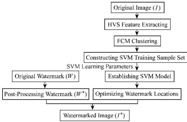
Fig. 1 Process of adaptive watermarking embedding.
